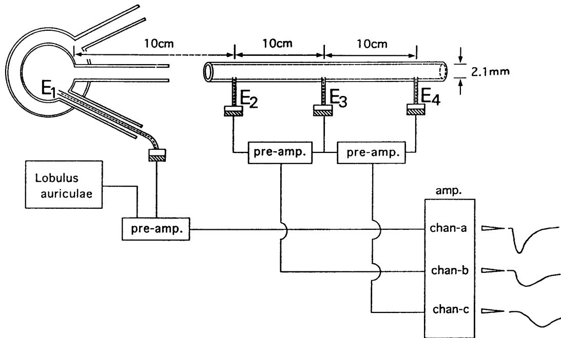
Fig. 1 Recording system and developed apparatus for parotid saliva. E_1 - E_4 : Thread electrode (thin vinyl tube with cotton thread inside filled with saline, and connected to Ag-AgCl electrode). pre-amp: Micro-electrode preamplifier (NIHON KOHDEN MEZ-7200).
