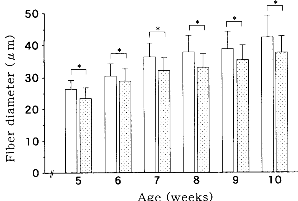
Fig.5 Effect of dietary consistency on fiber diameter in masseter muscles in rats of various ages. Open and dots bars indicate the pelleted diet group and the powdered group in rats. Each bar and its vertical line represent the mean and SD, respectively. * P < 0.001 .
