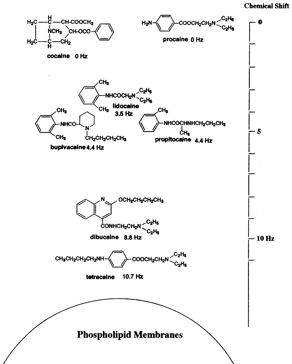
Fig.1 Proximity between phospholipid membrane and local anesthetics estimated by chemical shifts of choline methyl signal of phospholipid membrane. Lidocaine(3.5Hz), bupivacaine(4.4Hz), propitocaine(4.4Hz), dibucaine(8.8Hz) and tetracaine(10.7Hz).
