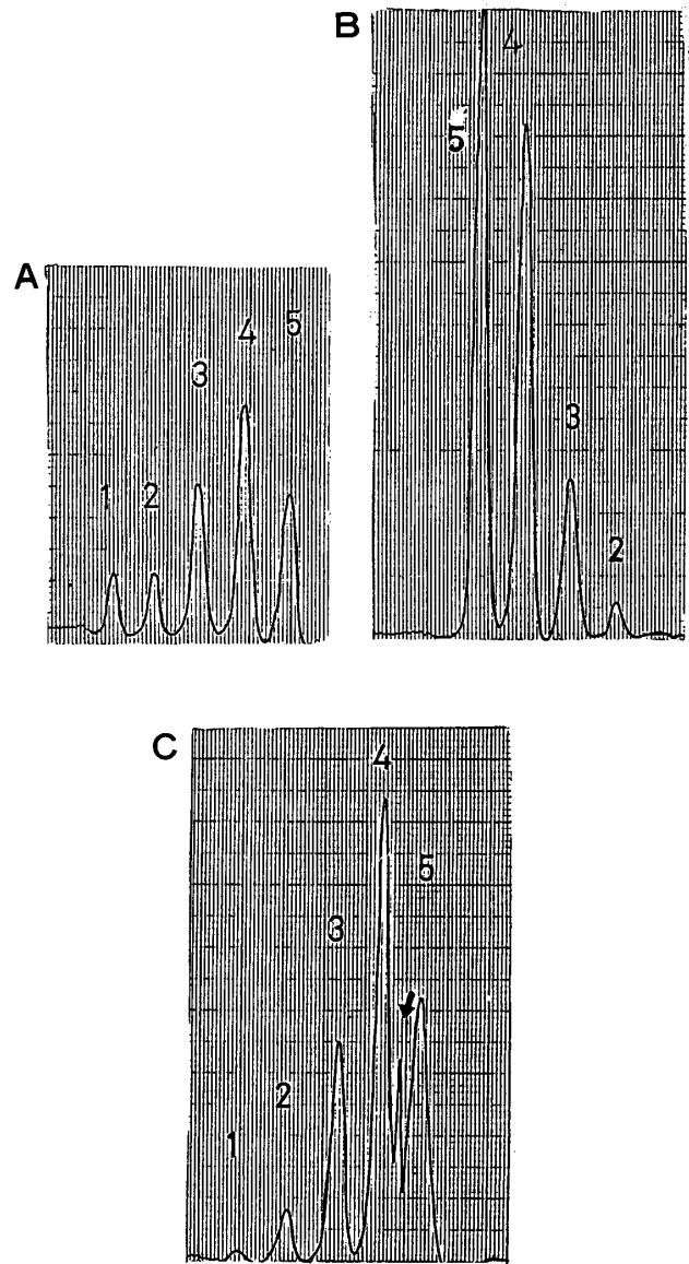
Fig. 2 Densitometer scanned LDH isozyme profiles. A. LDH isozyme pattern of normal human serum. B: LDH isozyme pattern of normal human parotid Saliva. C: LDH isozyme pattern of normal human whole saliva. The number at the top of each peak shows the relative location of the isozymes.
